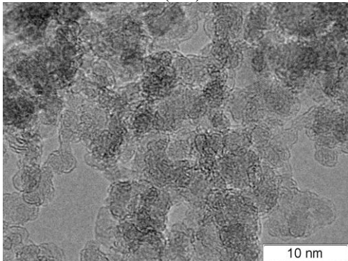
Fig. 7. Detonation nanodiamonds.
